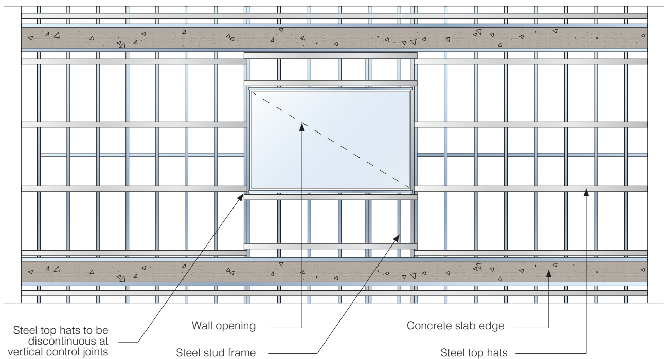
Fig 18. Typical Framing Arrangement Elevation
