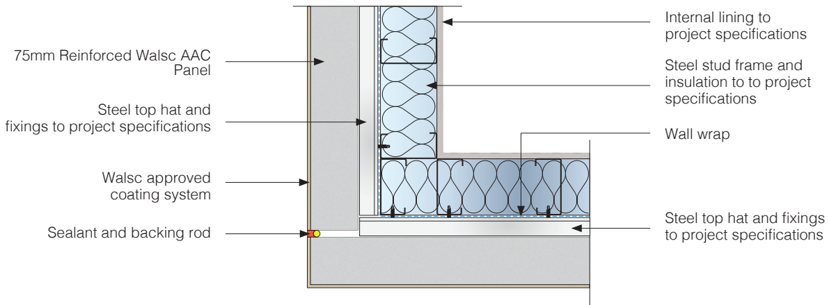
Fig 13. External Corner Control Joint Detail
