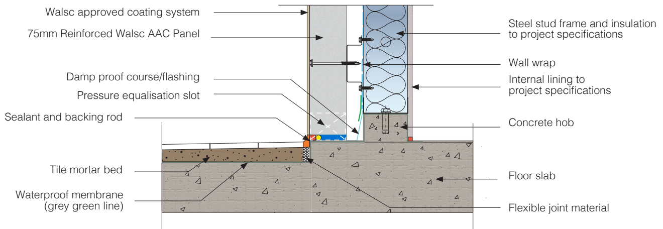
Fig 9. Balcony Step Down Detail 2
