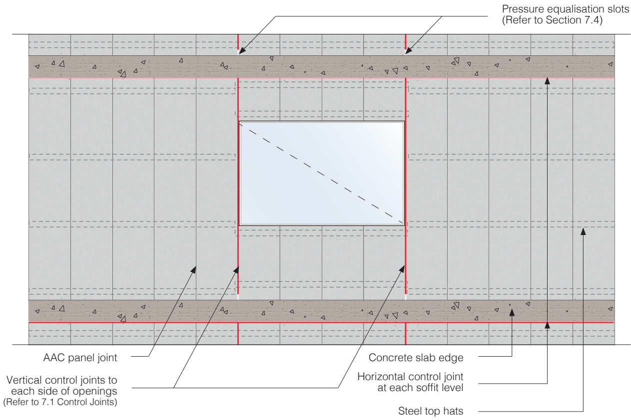
Fig 19. Typical Panel Arrangement Elevation
