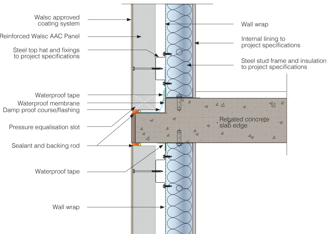
Fig 7. Rebated Slab Edge Detail
