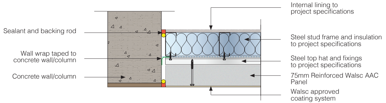
Fig 11. External Wall to Column Intersection Detail
