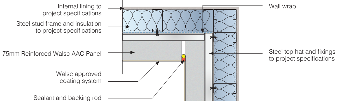
Fig 13. External Corner Control Joint Detail
