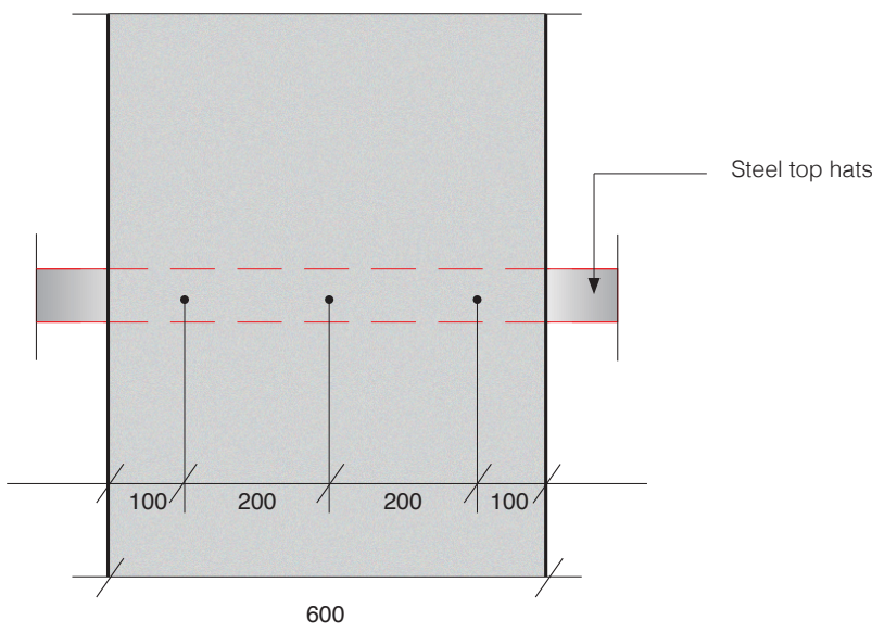
Fig 20. AAC Panel Fixing Detail
