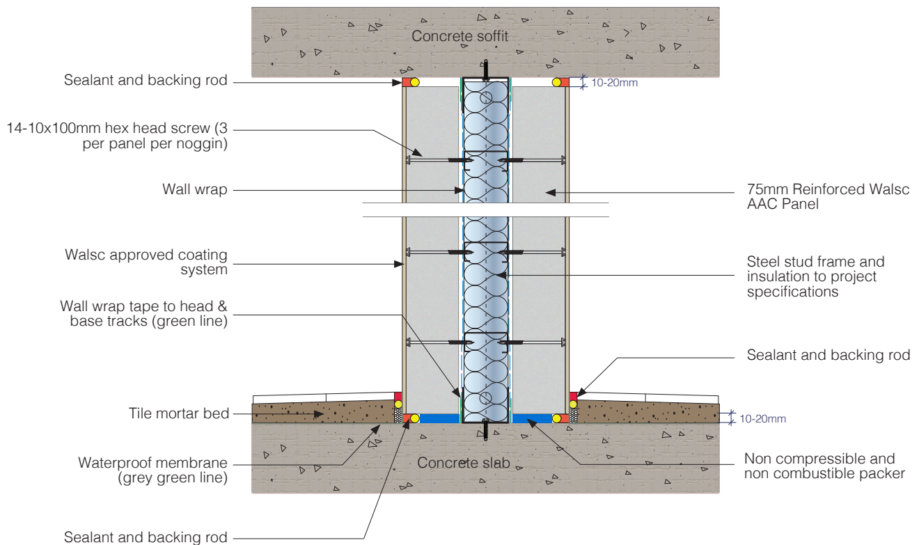
Fig 22. Head and Base Junctions Detail
