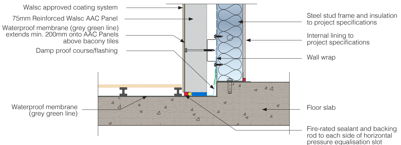
Fig 10. Balcony Step Down Detail 3
