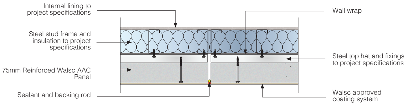
Fig 12. Vertical Control Joint Detail
