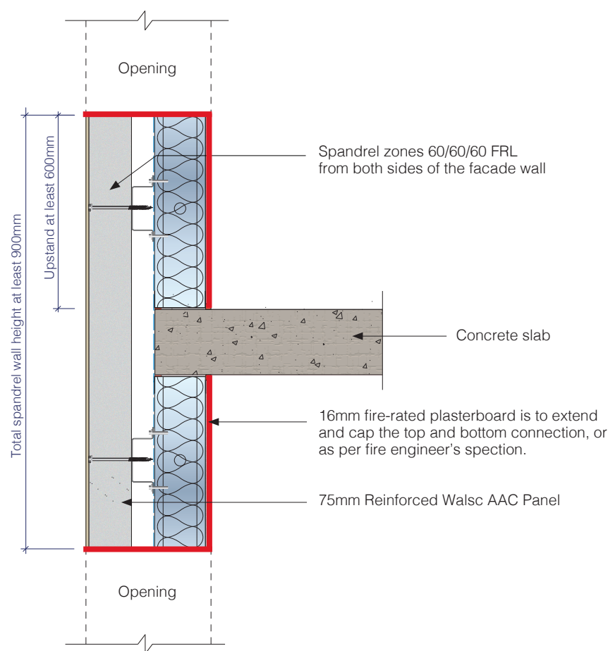
Fig 5. Walsc Vertical Spandrel Detail with Dimension
