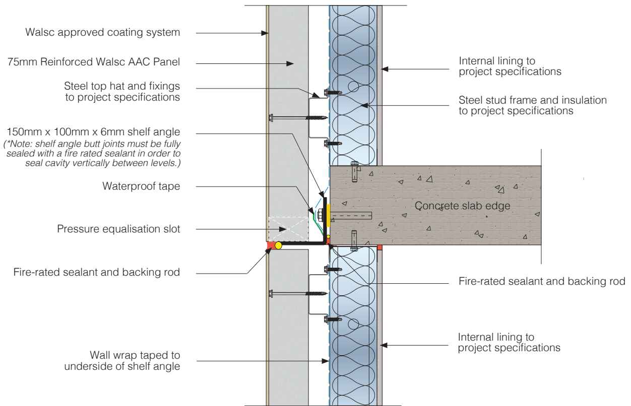
Fig 6. Unexposed Slab Edge Detail
