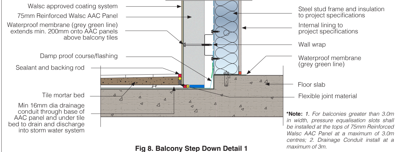
Fig 8. Balcony Step Down Detail 1
