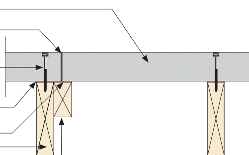
Fig 6. Panel End Joint Fixing Detail on Ledger Plate
