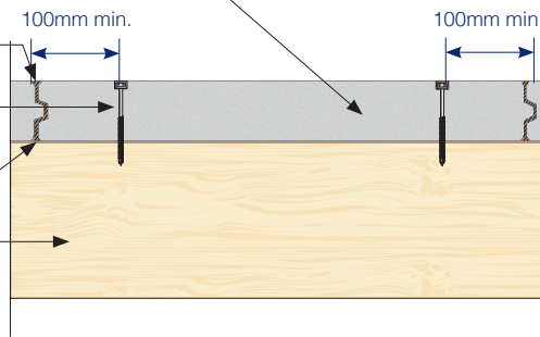
Fig 4. Fixing Detail
