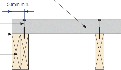
Fig 3. Edge Fixing Detail
