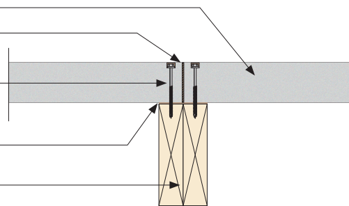
Fig 5. Panel End Joint Fixing Detail on Double Joist
