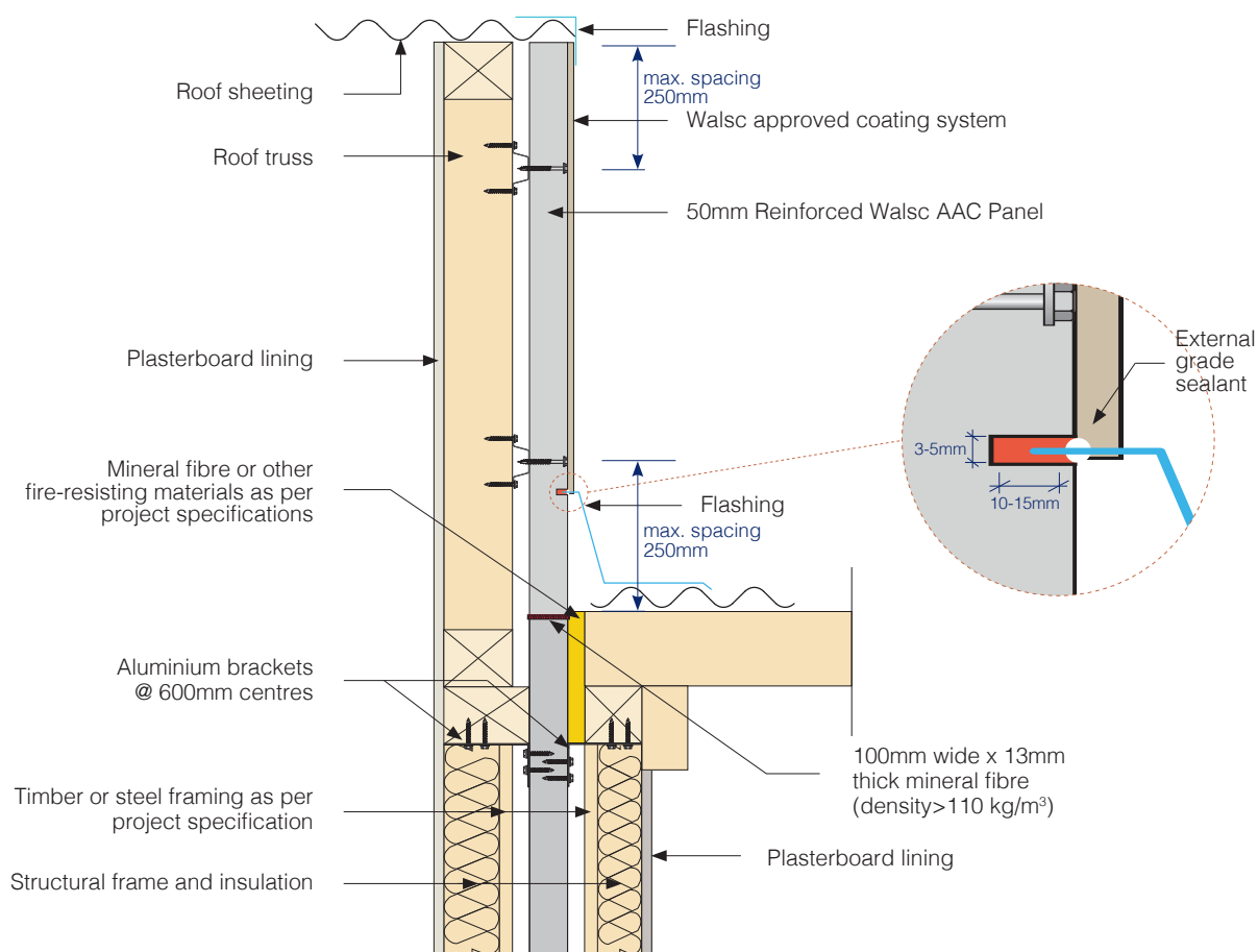
Fig 18. Vertically Aligned System Inter-tenancy Wall to External Walls Detail A
