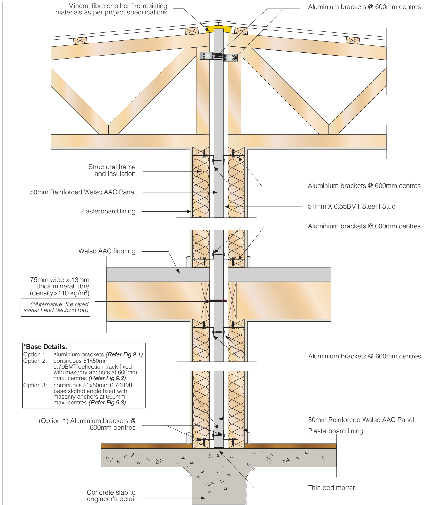
Fig 20. Horizontally Aligned System Cross Section
