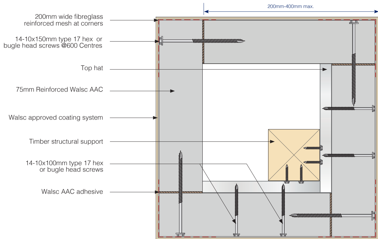
Fig 29. Column Top View Detail 1
