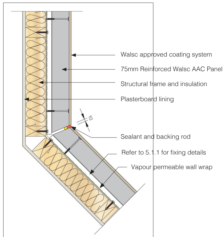
Fig 19. Internal Control Joint Detail 2
