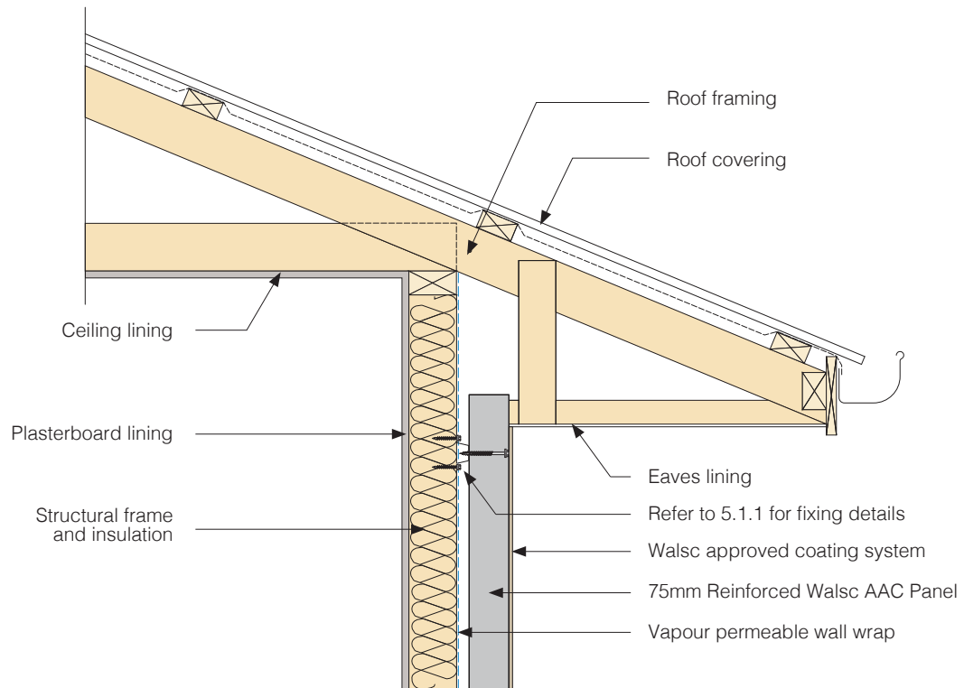
Fig 5. Eaves Detail 1
