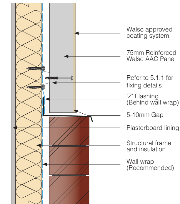
Fig 14. Conjunction detail between AAC Panel and Brick Veneer 1
