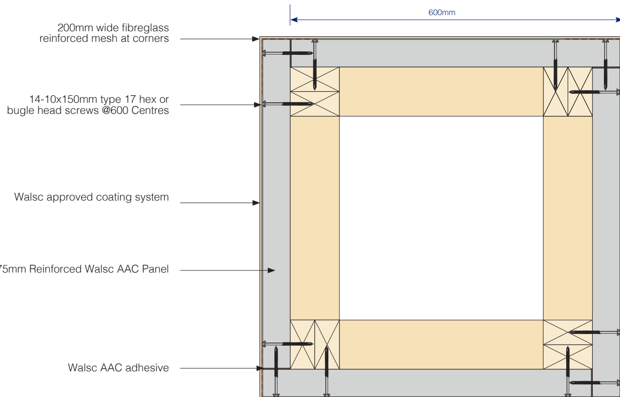
Fig 30. Column Top View Detail 2
