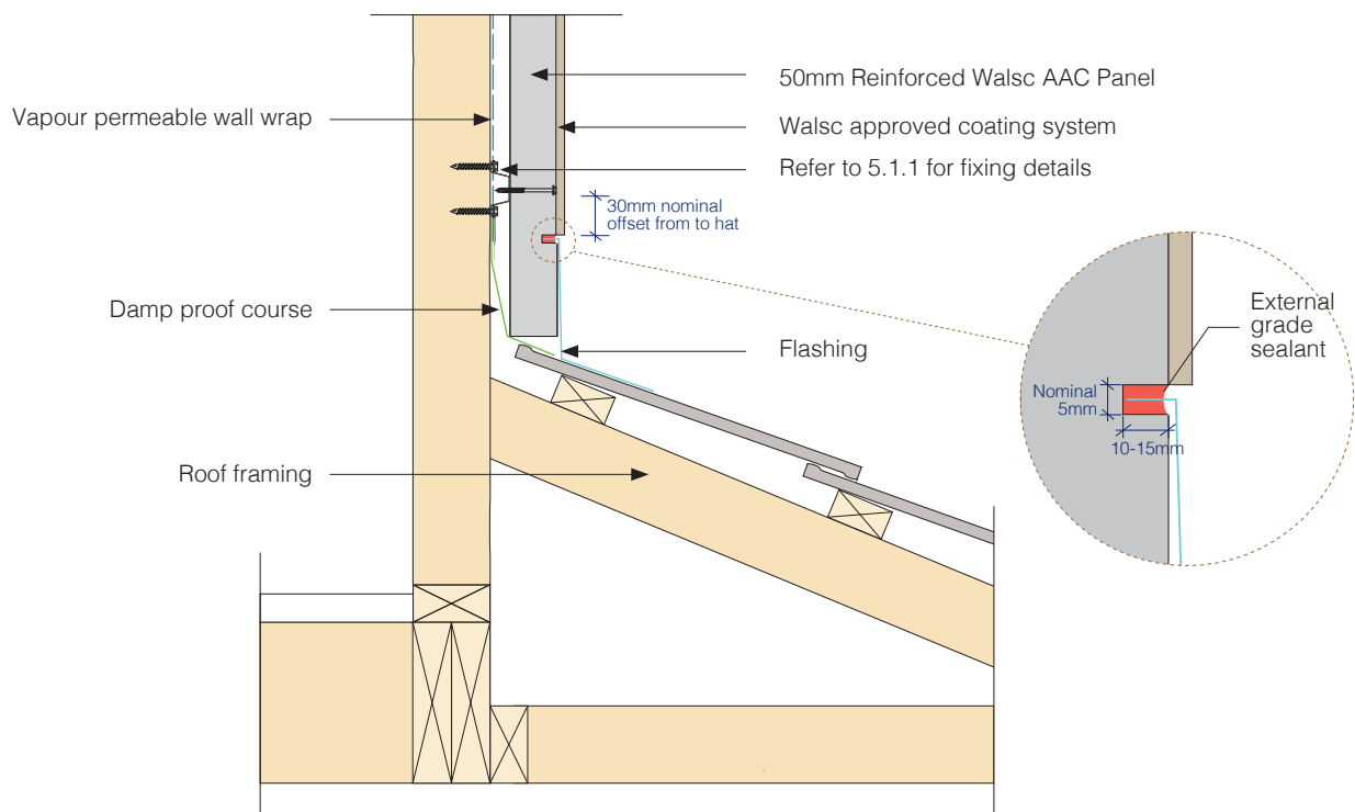
Fig 14. Panel to Roof Junction Detail (Option 1)
