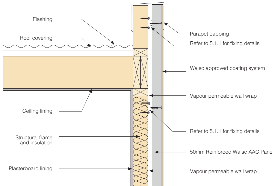
Fig 13. Parapet Wall Detail
