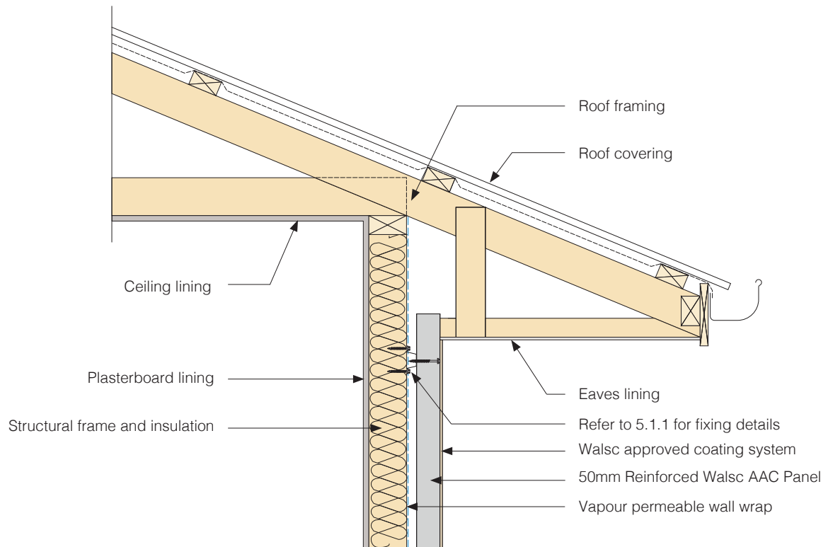
Fig 7. Eaves Detail 1
