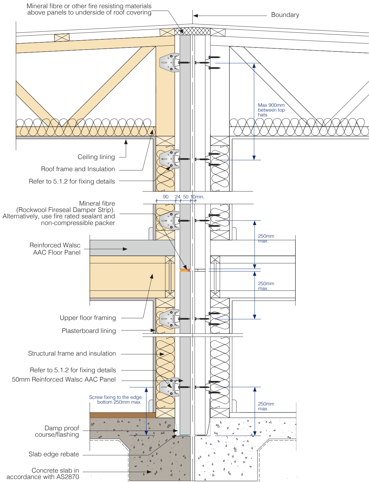
Fig 48. Boundary Wall Detail 2
