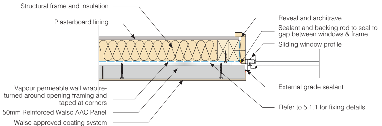
Fig 27. Window Jamb Detail
