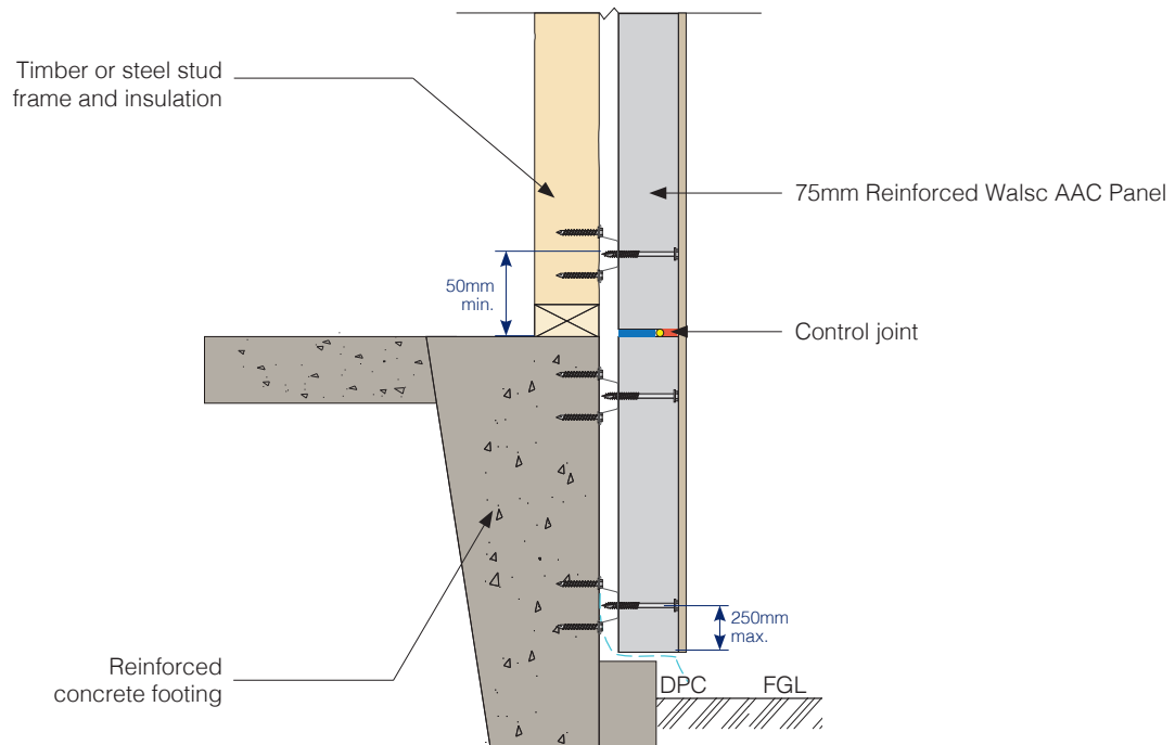
Fig 12. Junction to Deep Concrete Edge Beam
