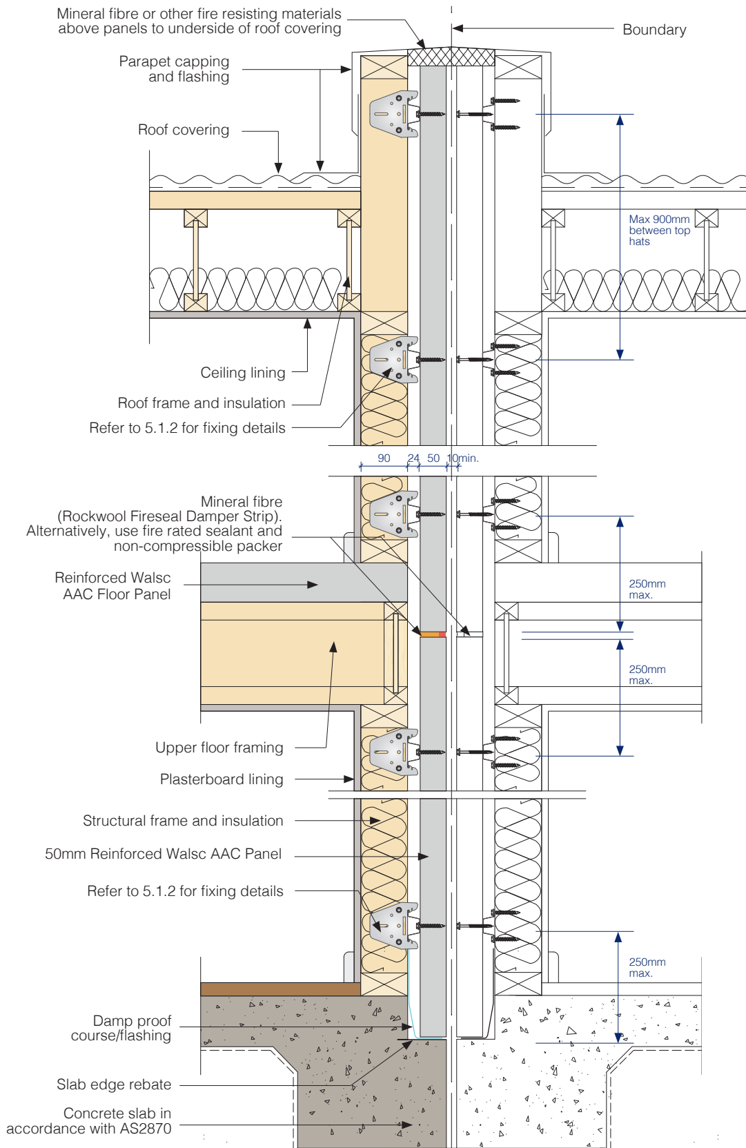
Fig 47. Boundary Wall Detail 1
