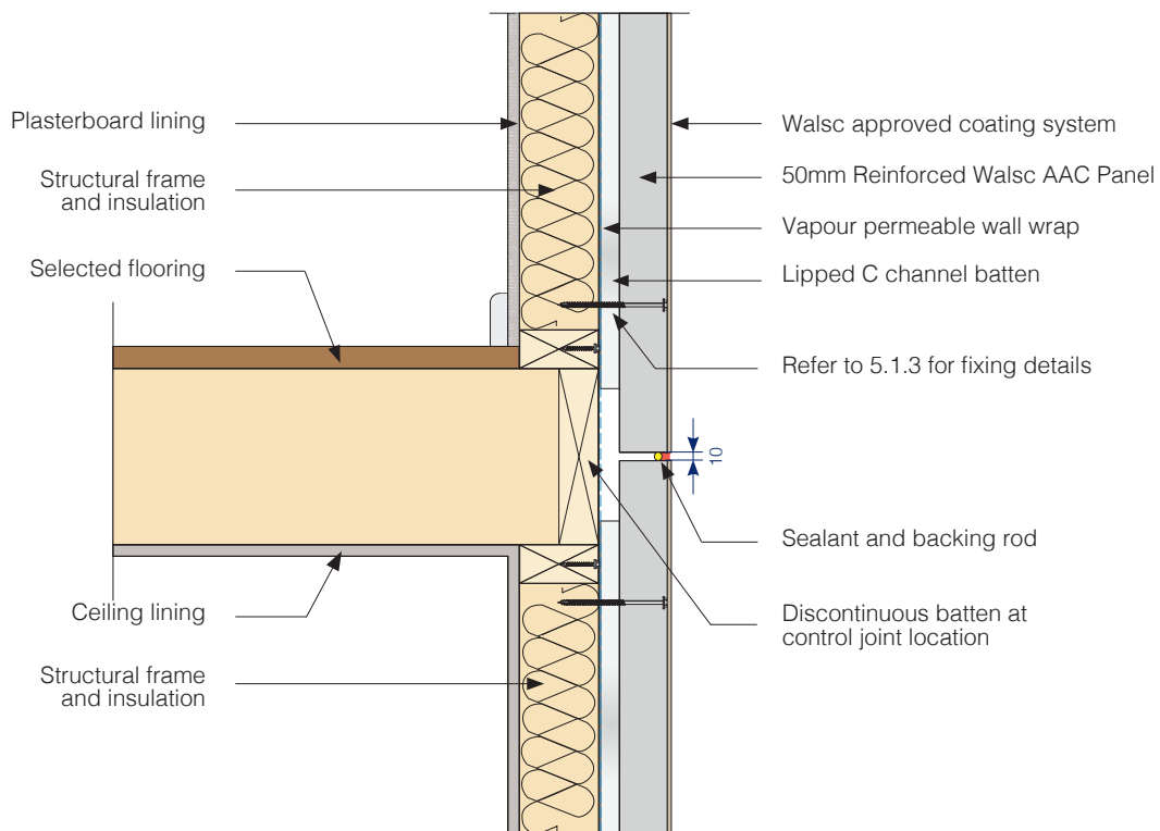
Fig 36. Inter-storey Junction Detail
