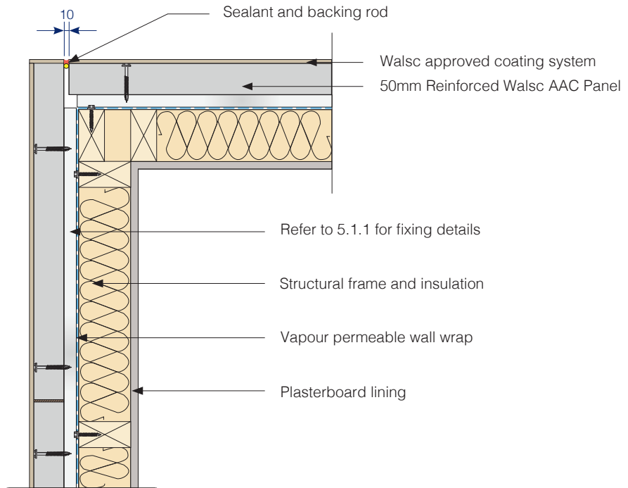
Fig 19. External Corner Joint Detail 1
