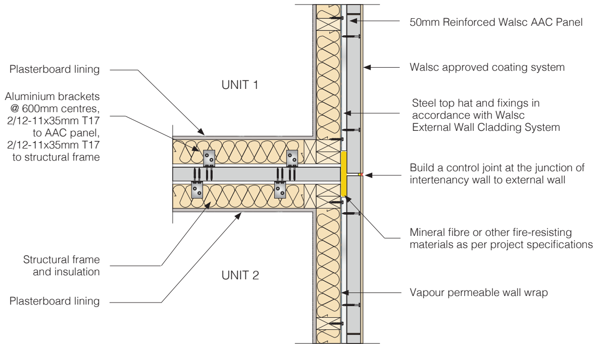
Fig 21. External Wall Junction Detail 1
