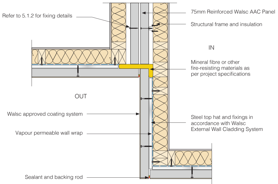
Fig 50. Boundary Wall Junction Detail 2
