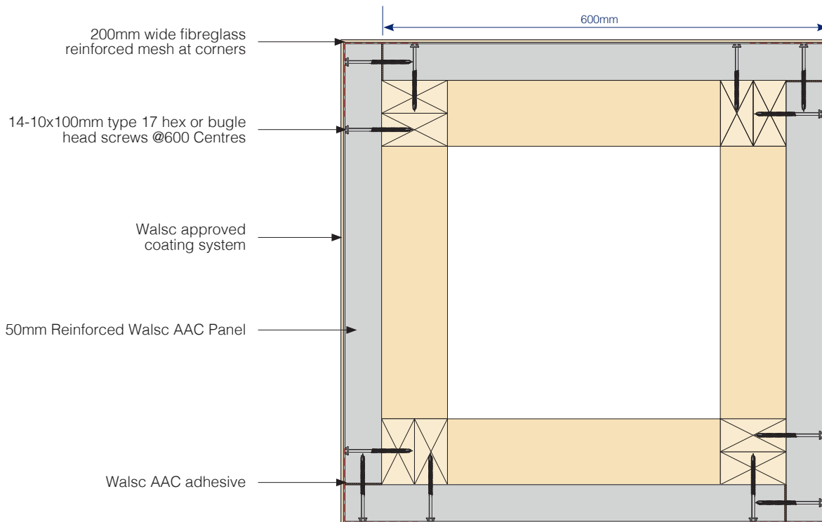
Fig 29. Column Top View Detail 2
