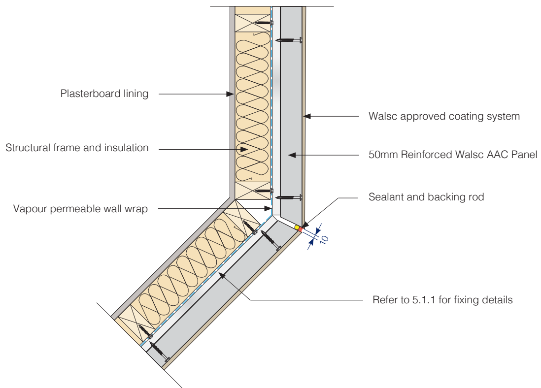
Fig 20. External Corner Joint Detail 2
