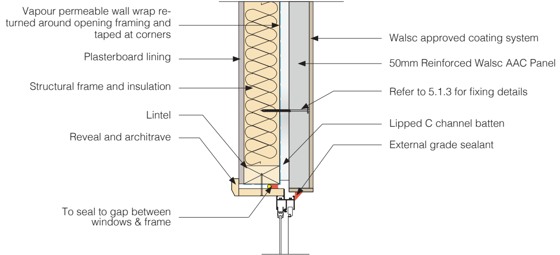
Fig 44. Window Head Detail
