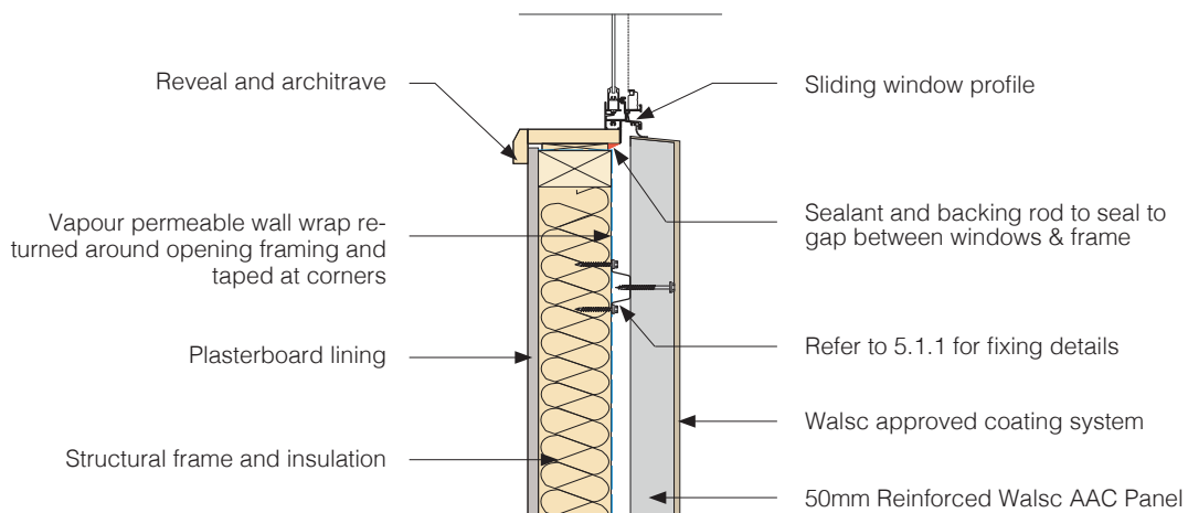
Fig 26. Window Sill Detail
