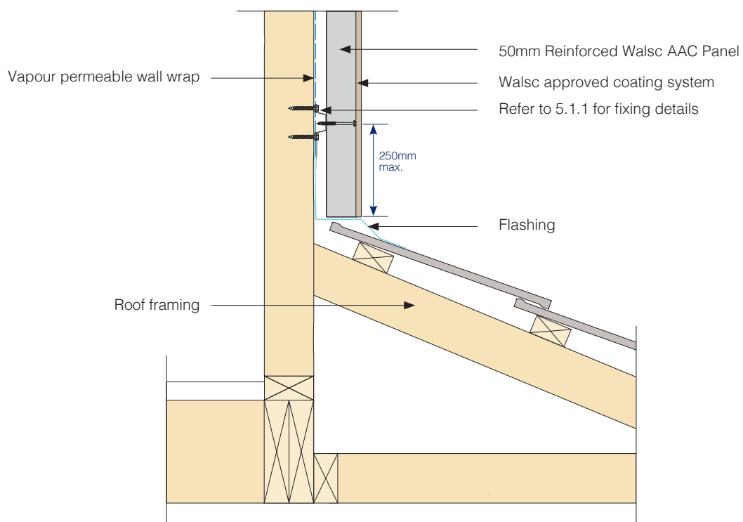
Fig 14.1 Panel to Roof Junction Detail (Option 2)
