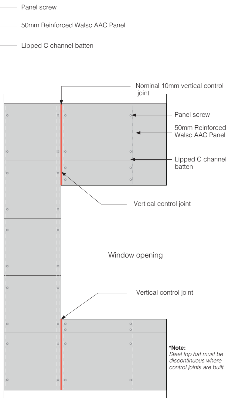
Fig 43. Horizontally Staggered System - Typical Opening with Control Joint Detail
