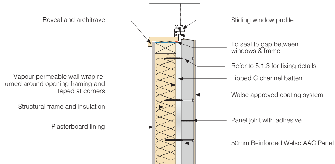
Fig 45. Window Sill Detail
