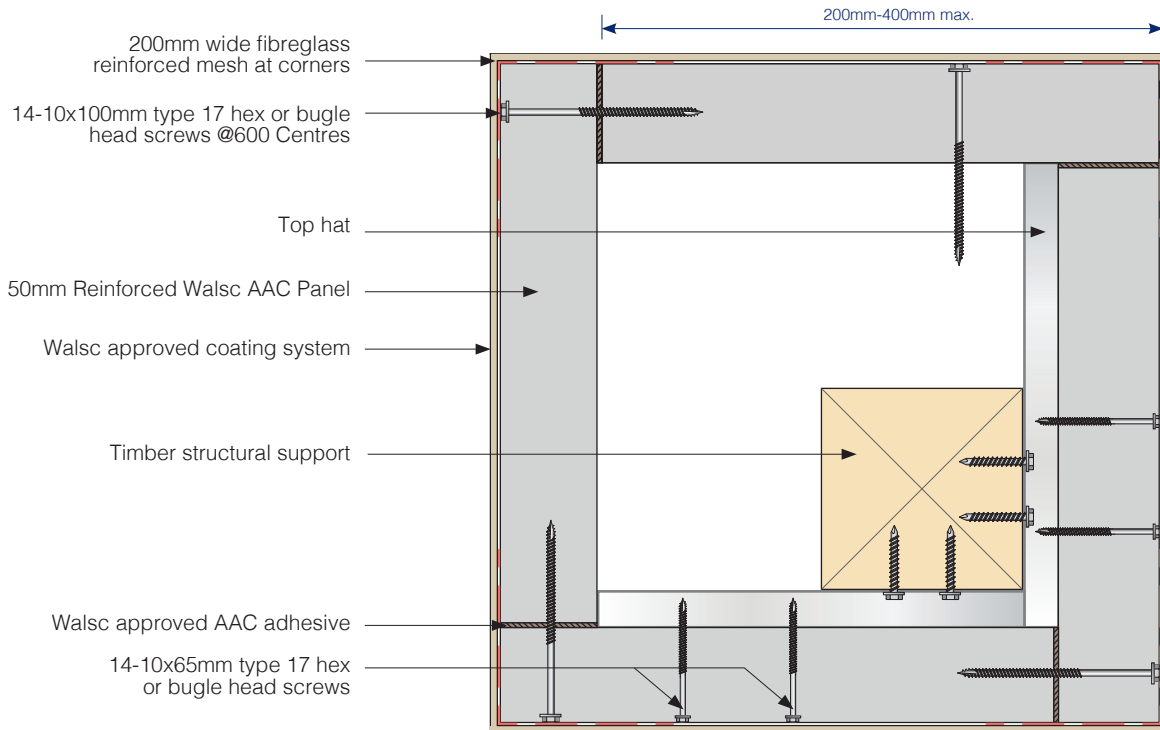
Fig 28. Column Top View Detail 1
