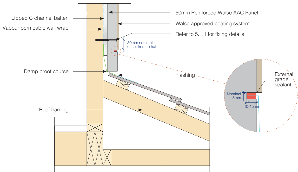
Fig 35. Panel to Roof Junction Detail
