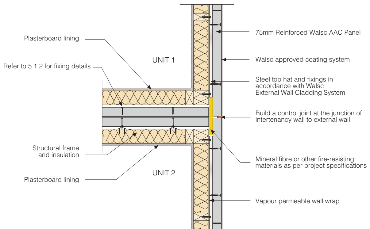
Fig 49. Boundary Wall Junction Detail 1
