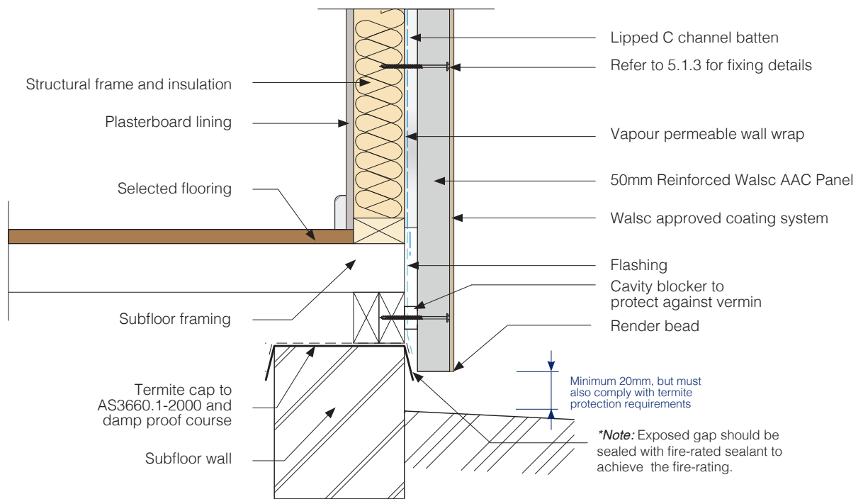
Fig 33. Suspended Floor Detail
