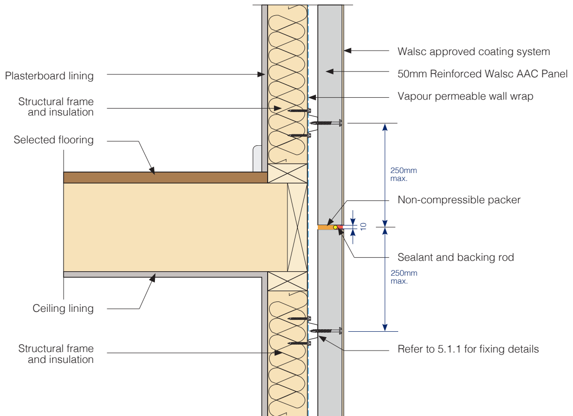
Fig 15. Inter-storey Junction Detail
