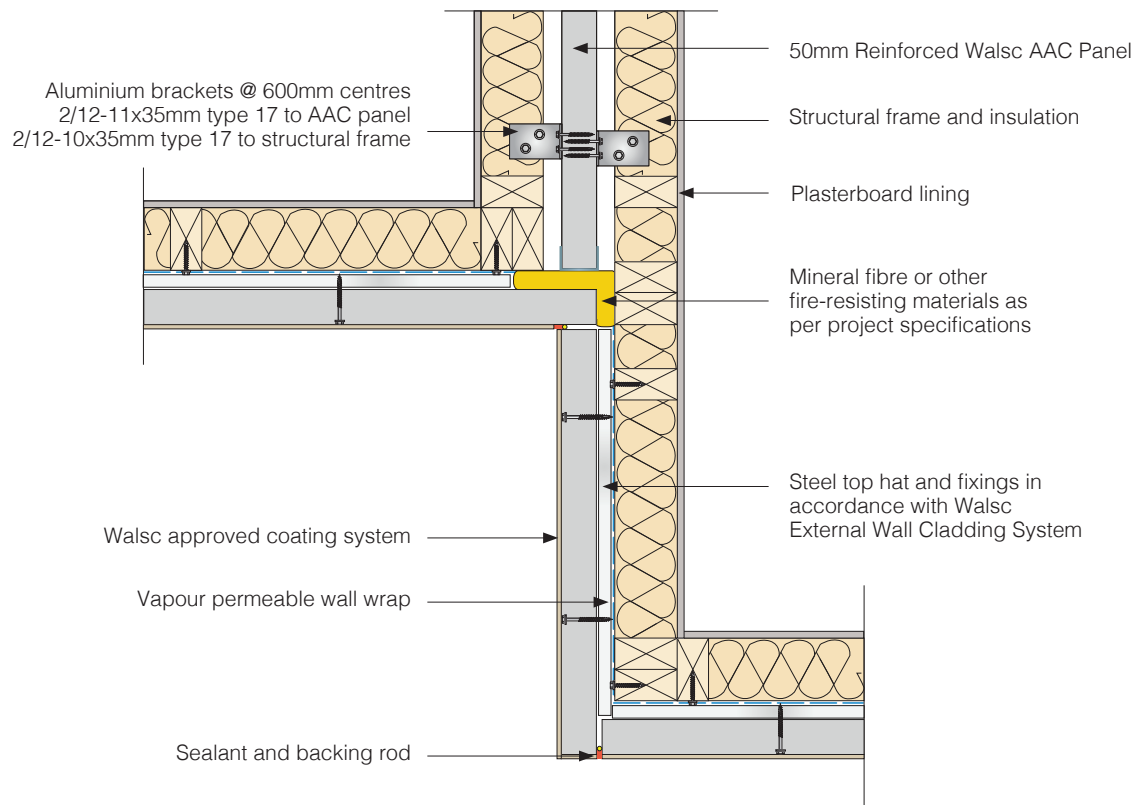
Fig 22. External Wall Junction Detail 2
