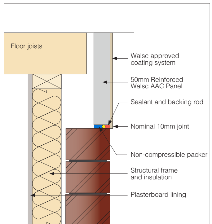
Fig 36. Inter-storey Junction Detail
