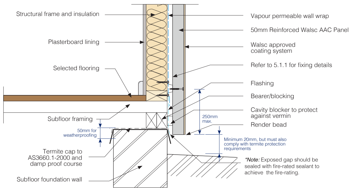
Fig 10. Suspended Floor Detail
