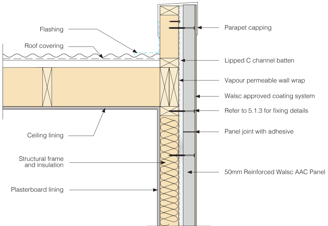
Fig 34. Parapet Wall Detail
