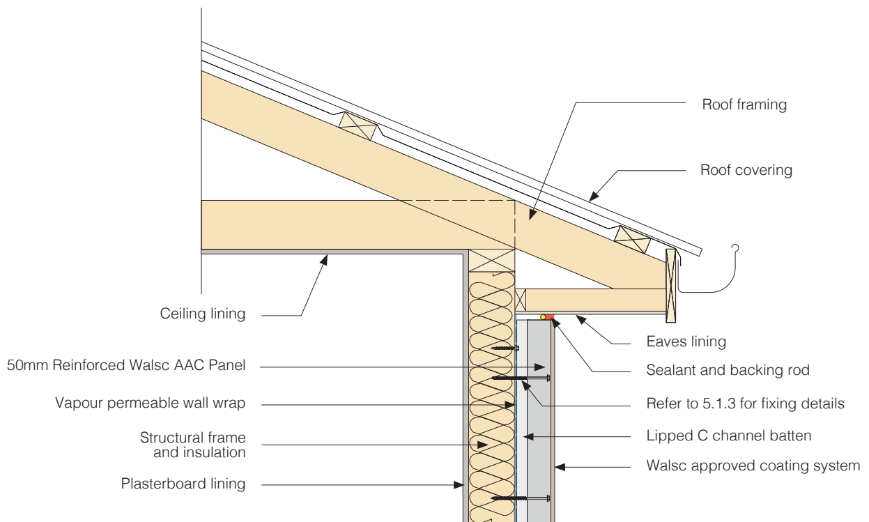
Fig 31. Eaves Detail 2
