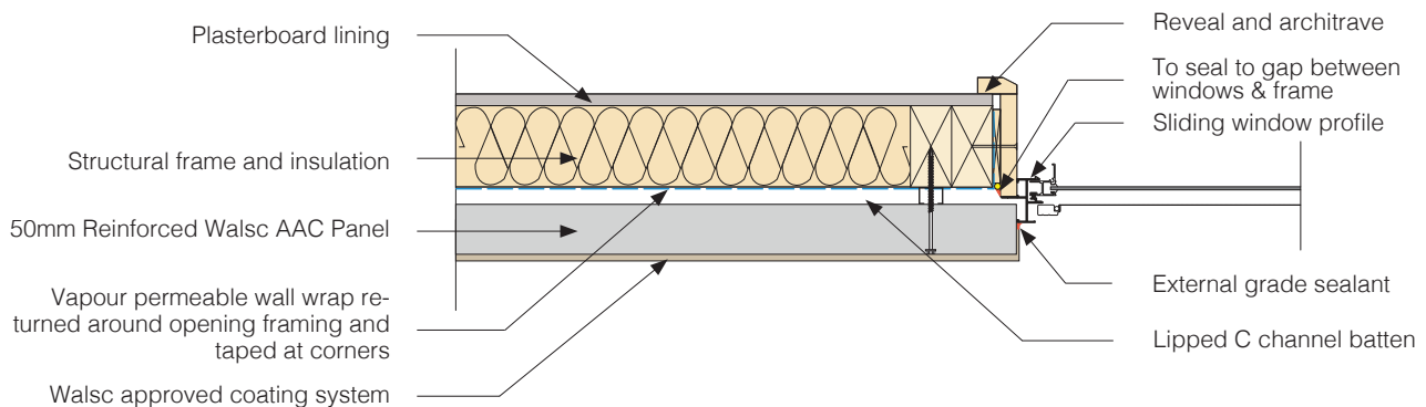
Fig 46. Window Jamb Detail
