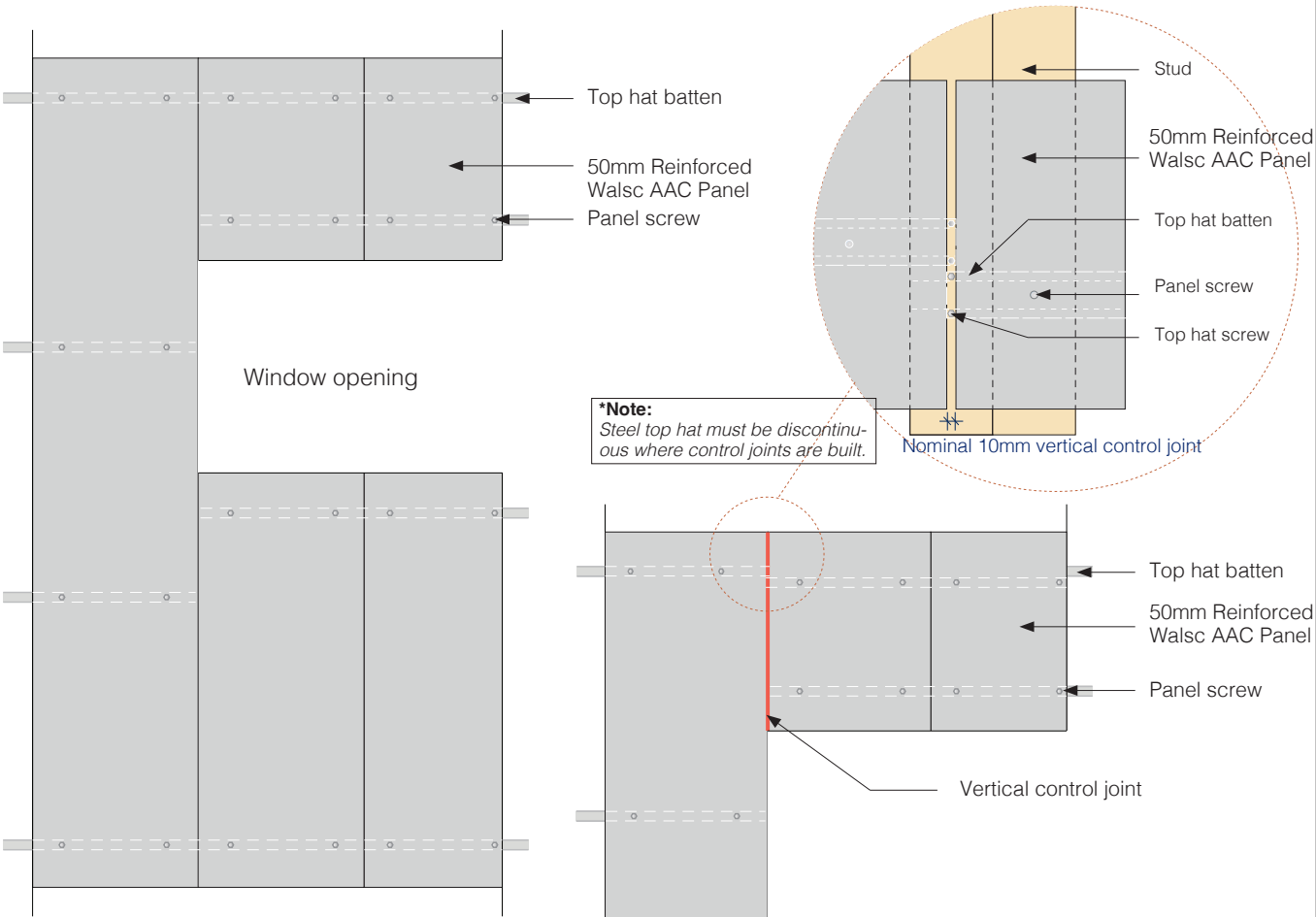
Fig 23. Vertical Aligned System -Typical Opening without Control Joint Detail
