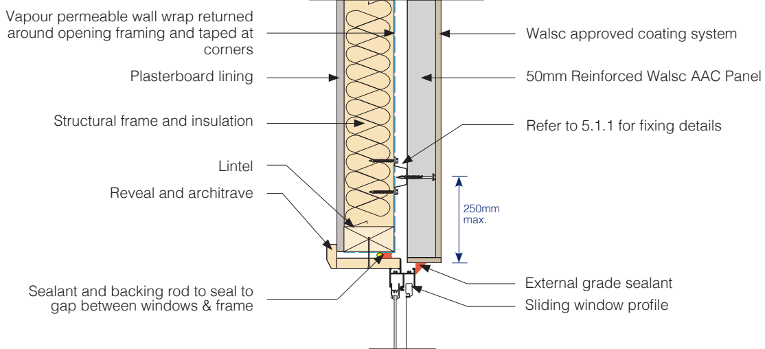
Fig 25. Window Head Detail
