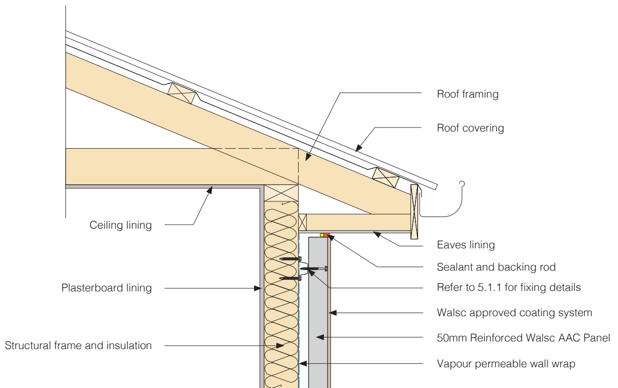
Fig 8. Eaves Detail 2
