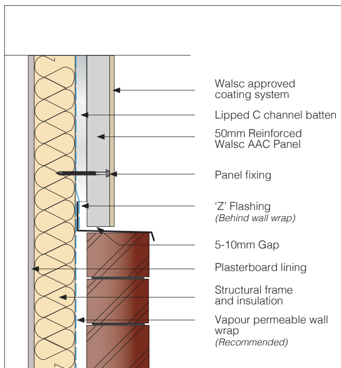
Fig 36. Inter-storey Junction Detail
