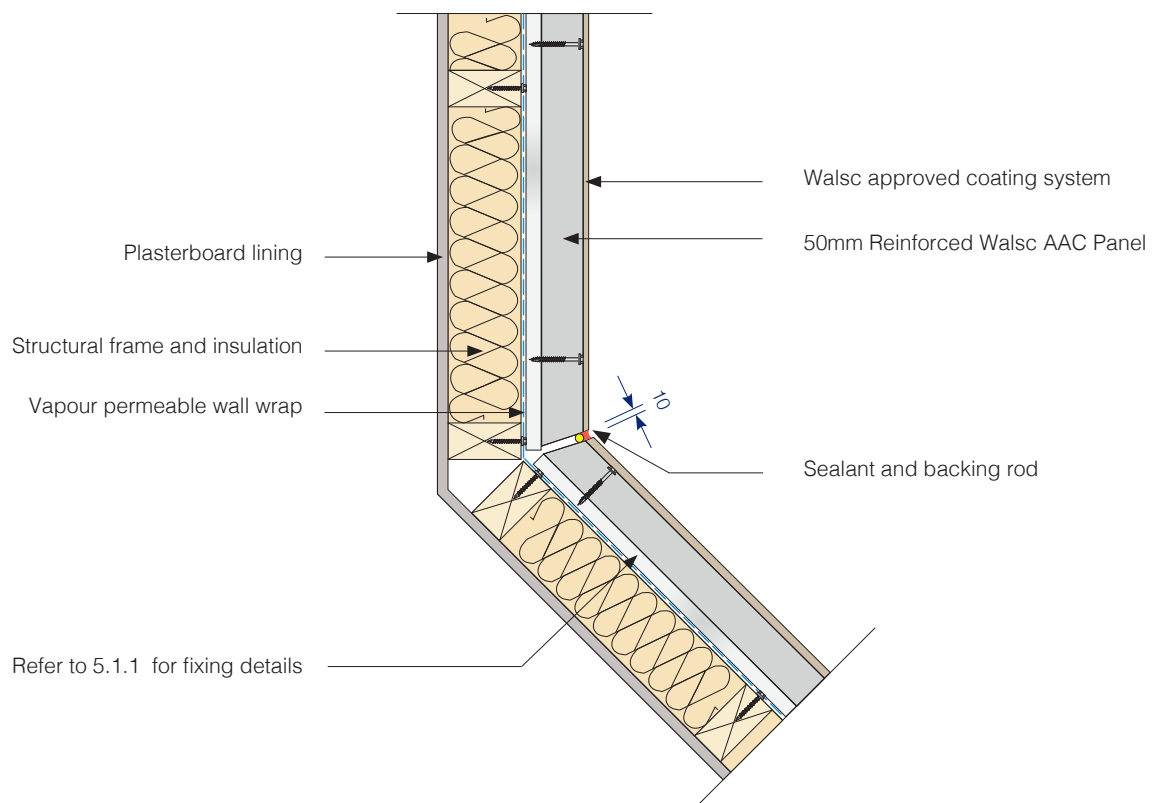
Fig 18. Internal Corner Joint Detail 2
