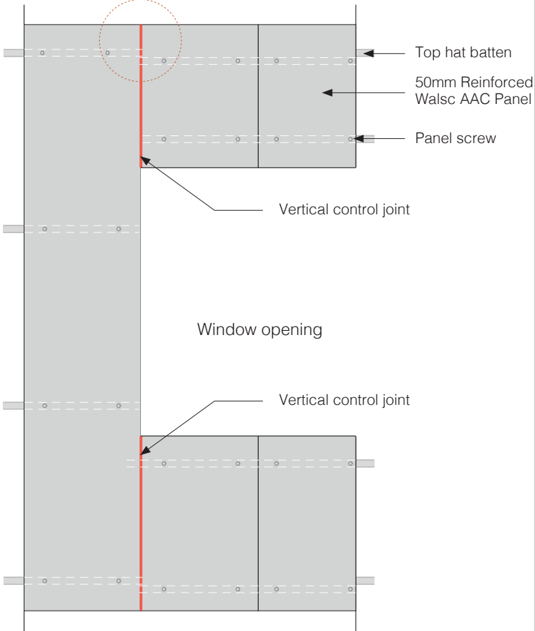
Fig 24. Vertical Aligned System - Typical Opening with Control Joint Detail
