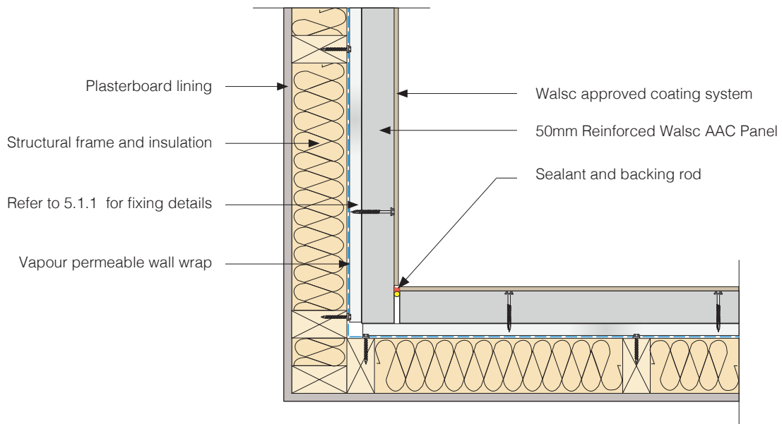
Fig 17. Internal Corner Joint Detail 1
