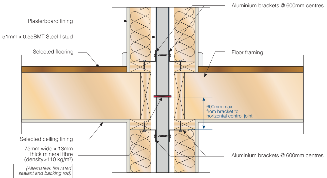
Fig 24. Horizontally Aligned System Inter-storey Junction Detail 1
