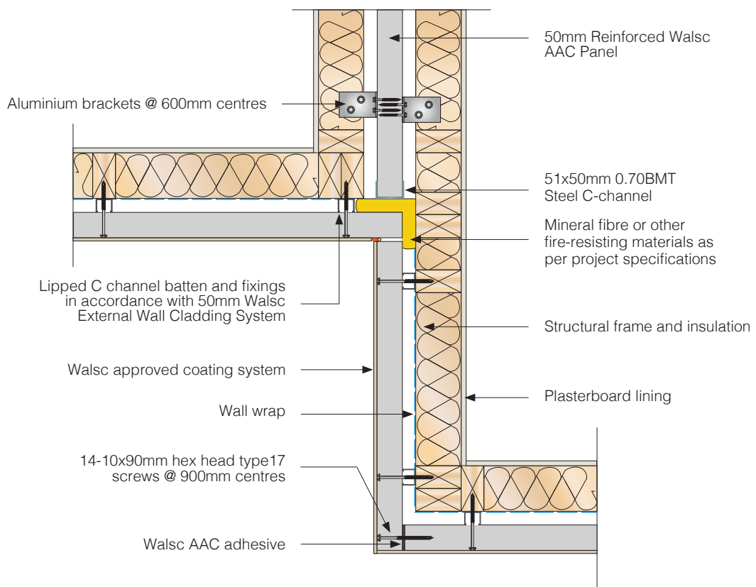
Fig 27. Horizontally Aligned System External Wall Junction Detail
