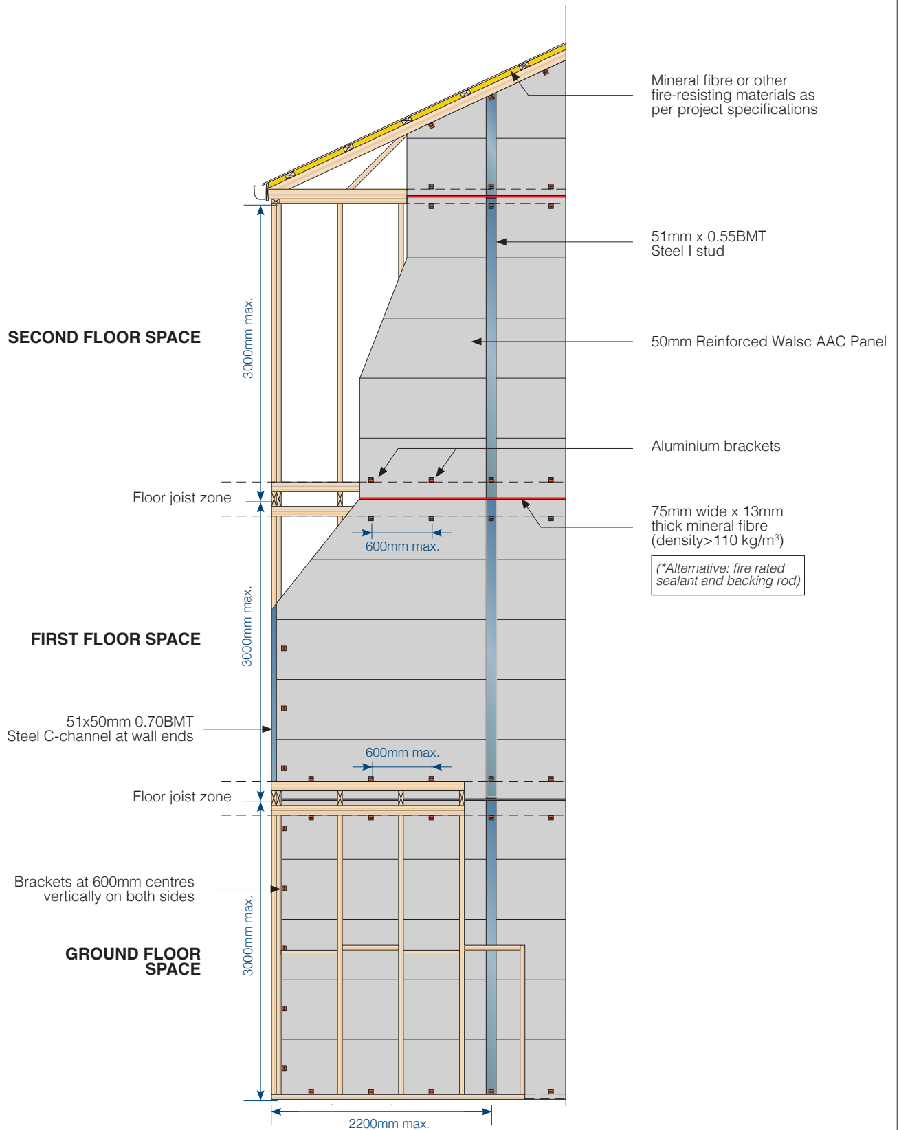
Fig 23. Horizontally Aligned System Panel Orientation Elevation with Inter-storey Junction Detail
