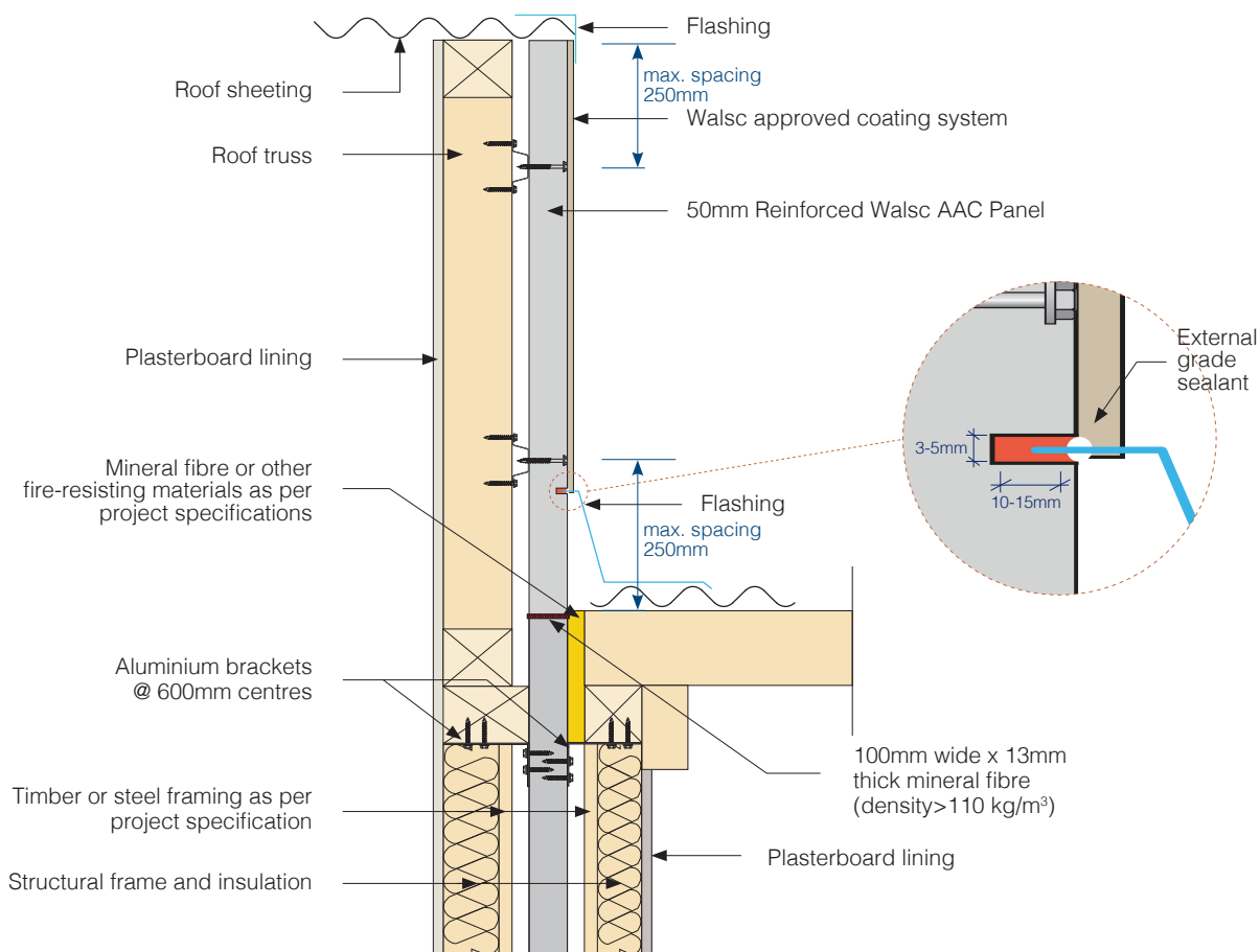
Fig 18. Vertically Aligned System Intertency Wall to External Walls Detail A
