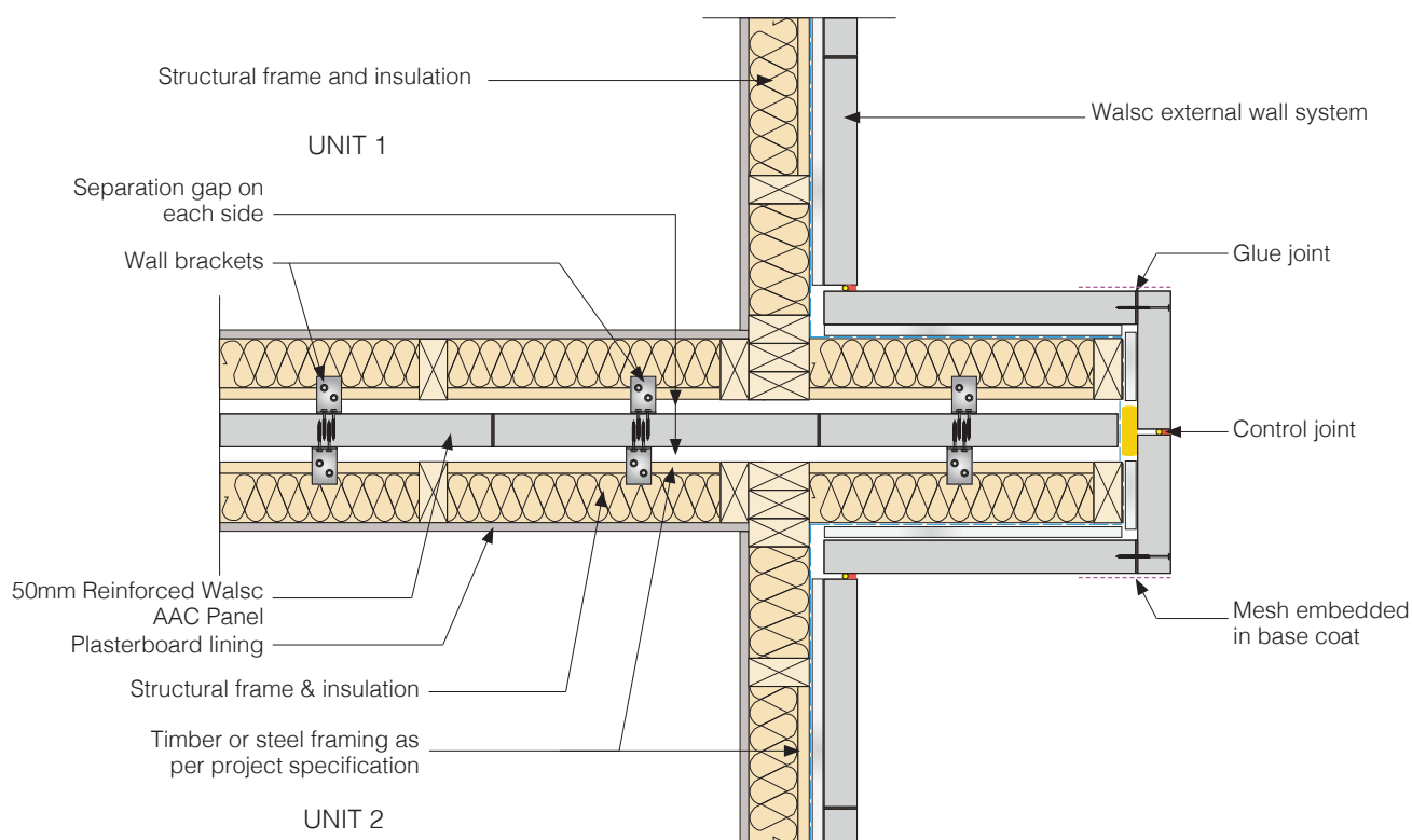
Fig 14. Nib junction detail of Walsc AAC Panel (50) Intertency wall & External Wall System
