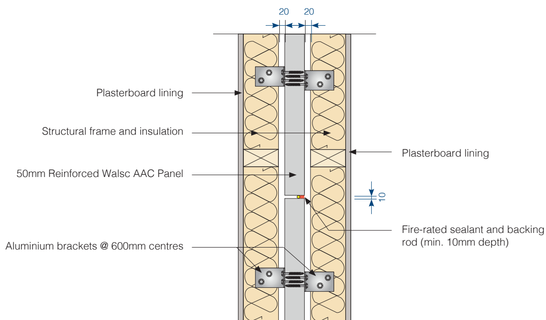
Fig 15. Vertically Aligned System Vertical Control Joint Detail
