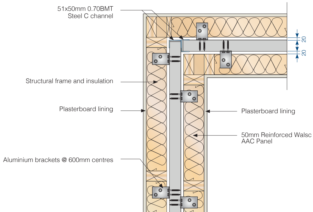
Fig 26. Horizontally Aligned System Corner Detail
