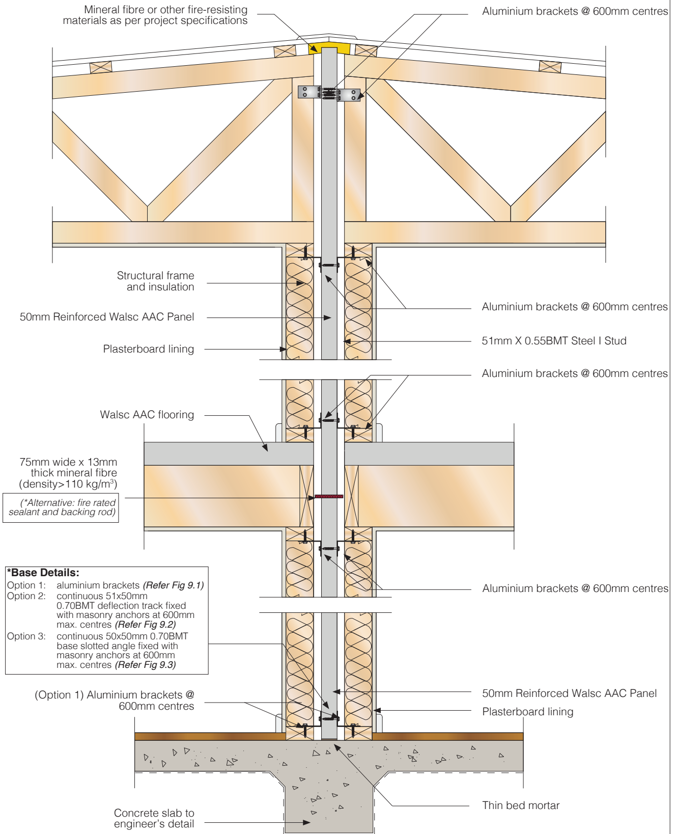
Fig 22. Horizontally Aligned System Cross Section
