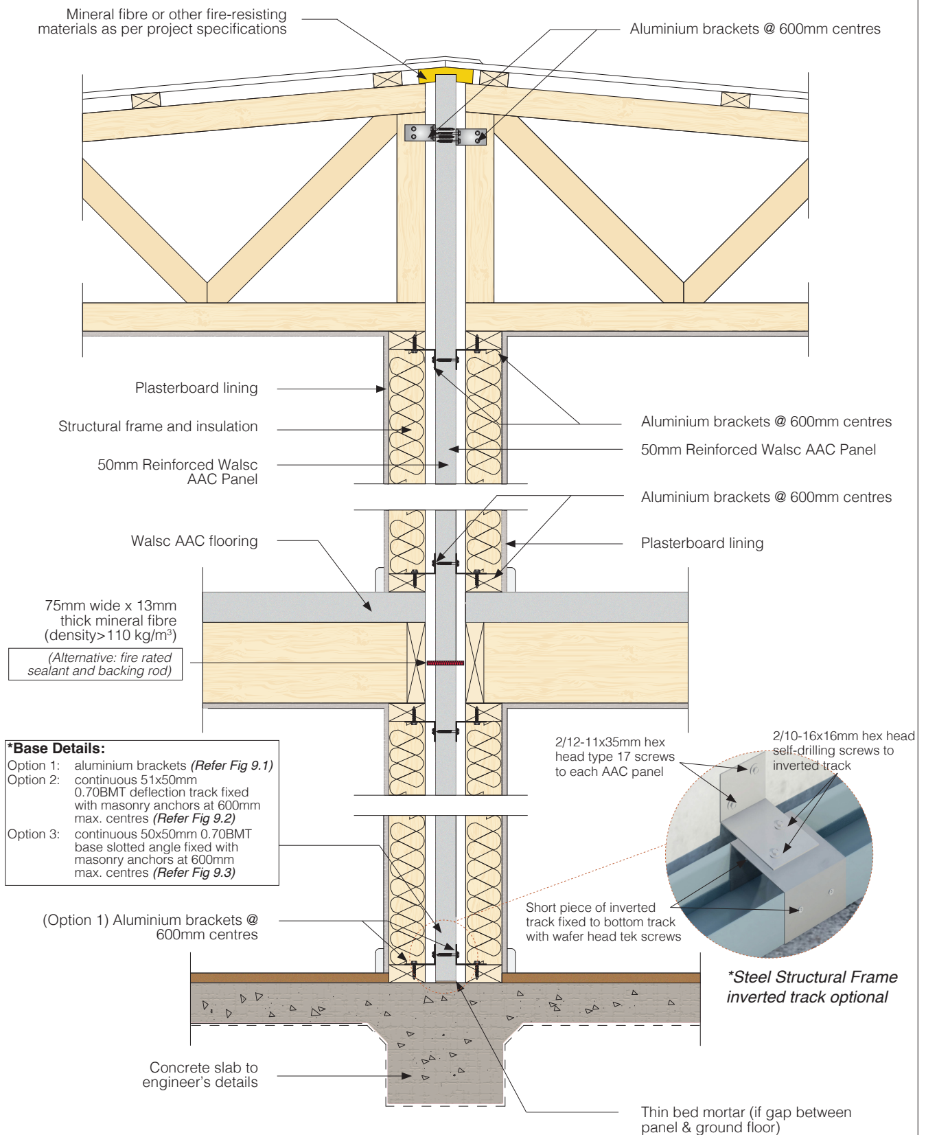
Fig 5. Vertically Aligned System Cross Section Detail
