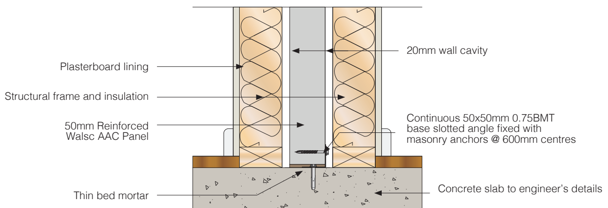
Fig 9.1 Vertically Aligned System Base of Wall Detail - Option 1
