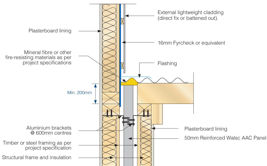
Fig 19. Vertically Aligned System Intertency Wall to External Walls Detail B
