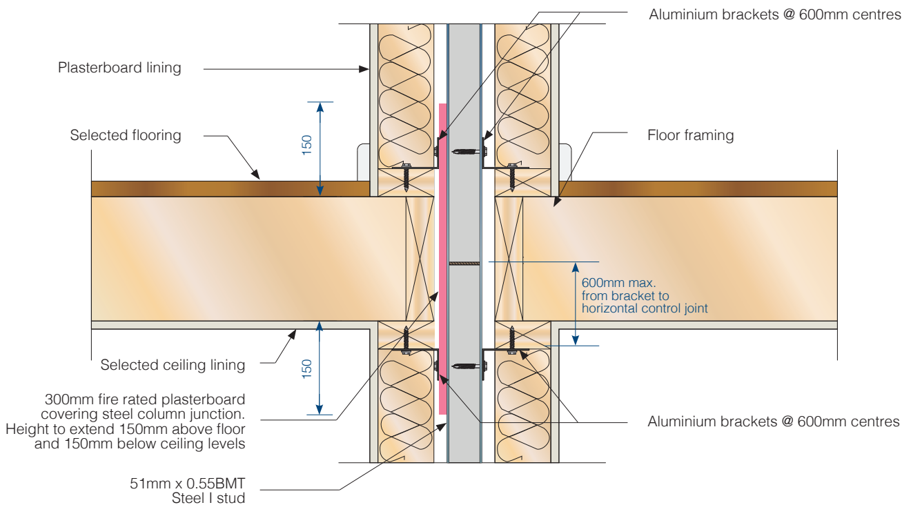
Fig 25. Horizontally Aligned System Inter-storey Junction Detail 2
